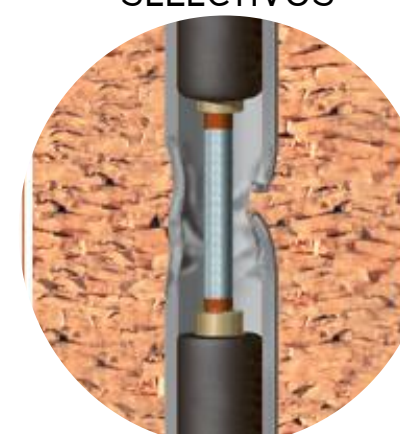
SCAB LINER
